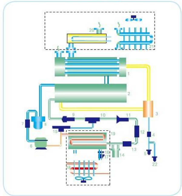
冷干机工艺流程 Process flow chat of refrigerated air dryer
